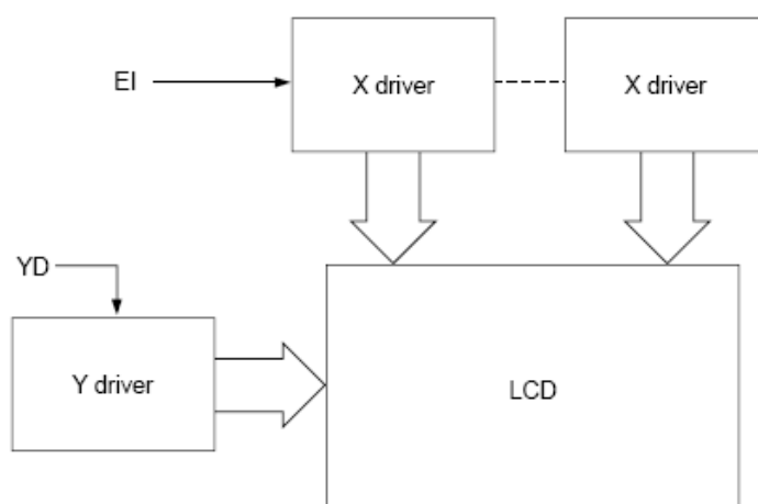
Figure 2. Single-panel display
