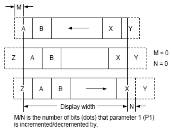
Figure 21. Horizontal scrolling
