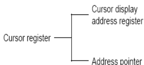
Figure 34. Cursor addressing
