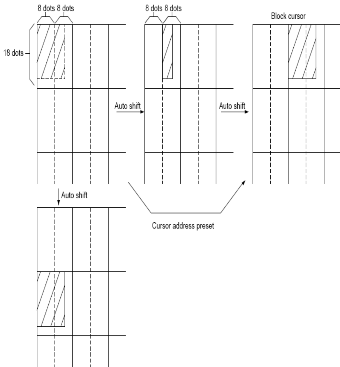
Figure 36. Cursor movement
