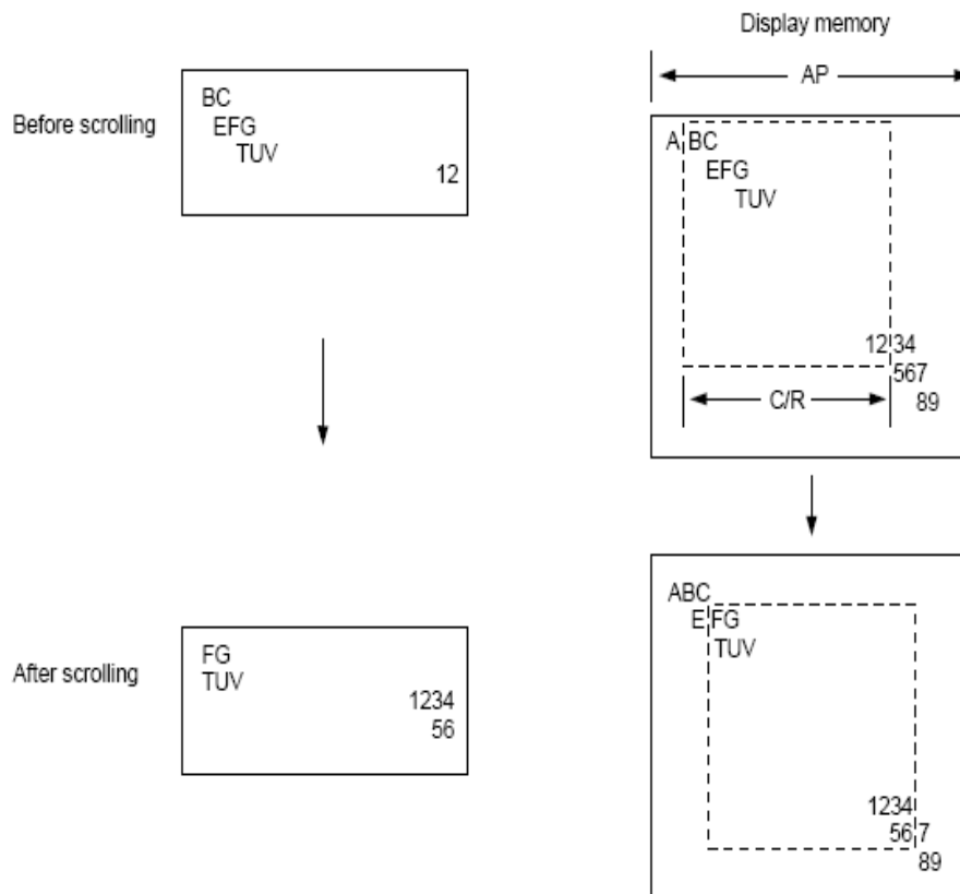
Figure 43. Bidirectional scrolling
