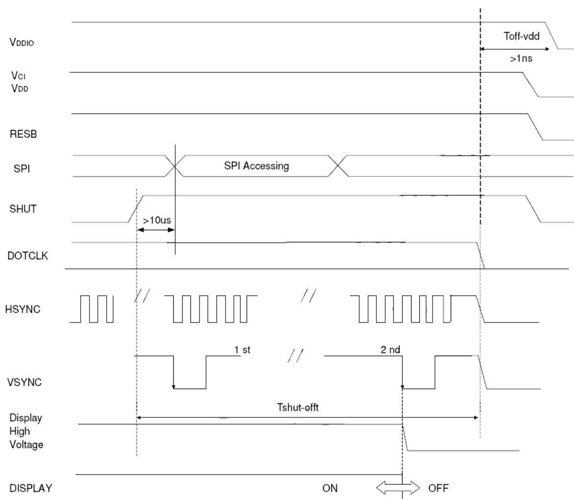
Figure 14. 11 Power Down Sequence
