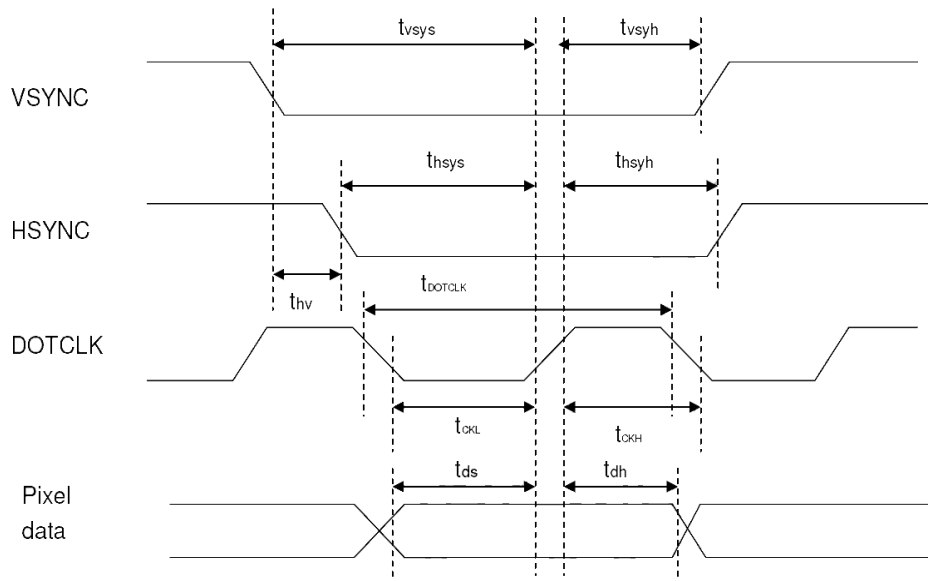
Figure 14. 1 Pixel Timing
