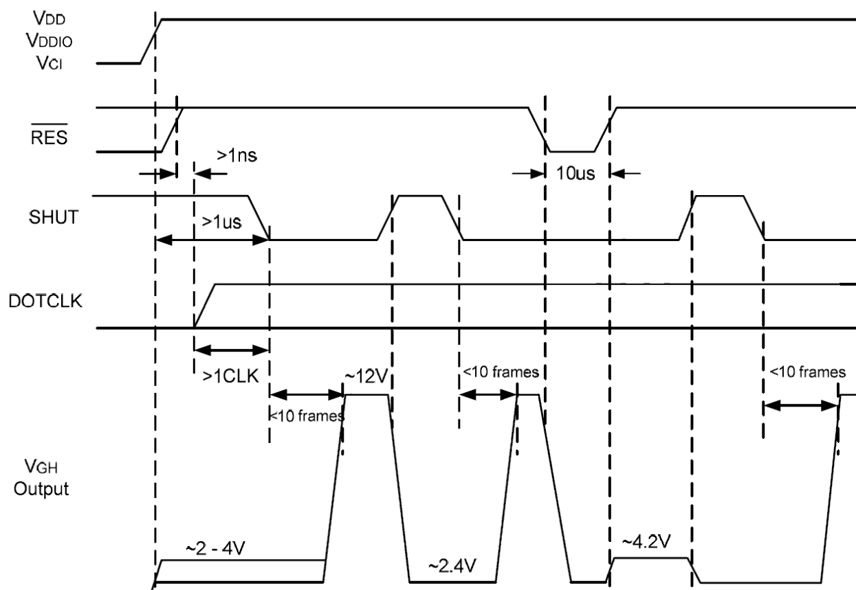
Figure 14. 9 VGH Output Against SHUT & RES
