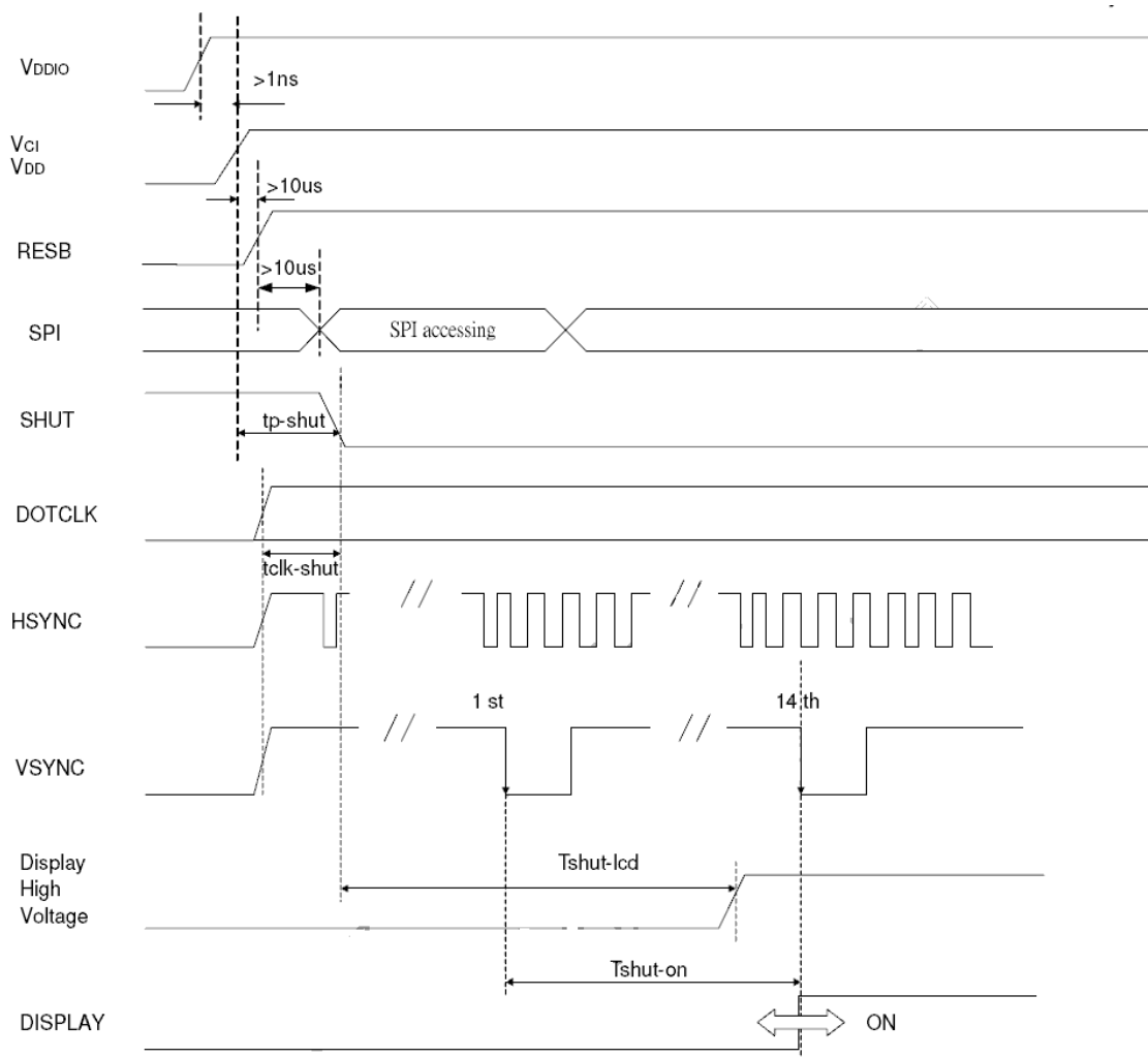
Figure 14. 10 Power Up Sequence
