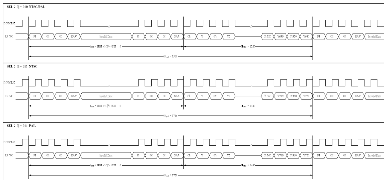
Figure 14. 7 CCIR656 horizontal timing
