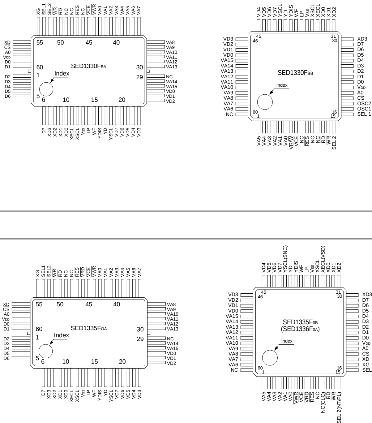
Figure 3. SED1330F and SED1335F pinouts
